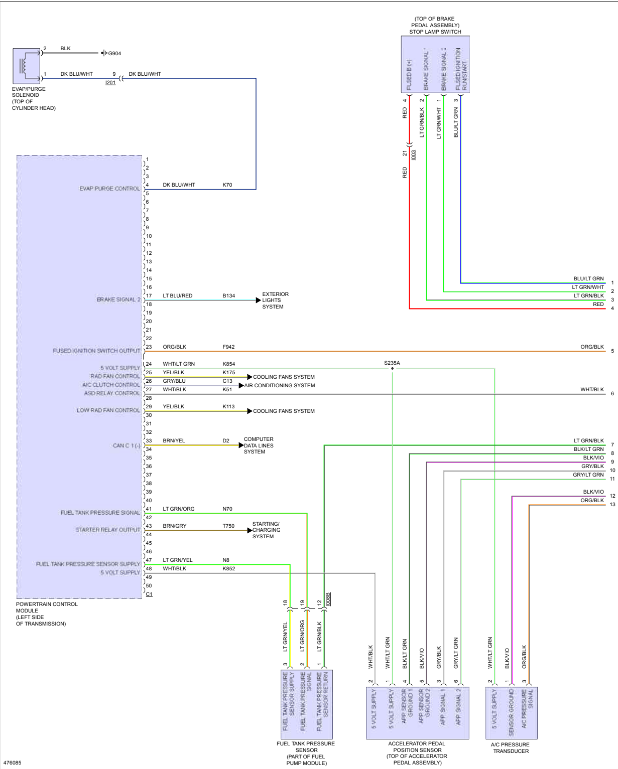
Fig 1: 2.4L, Engine Performance Circuit (1 of 6)
