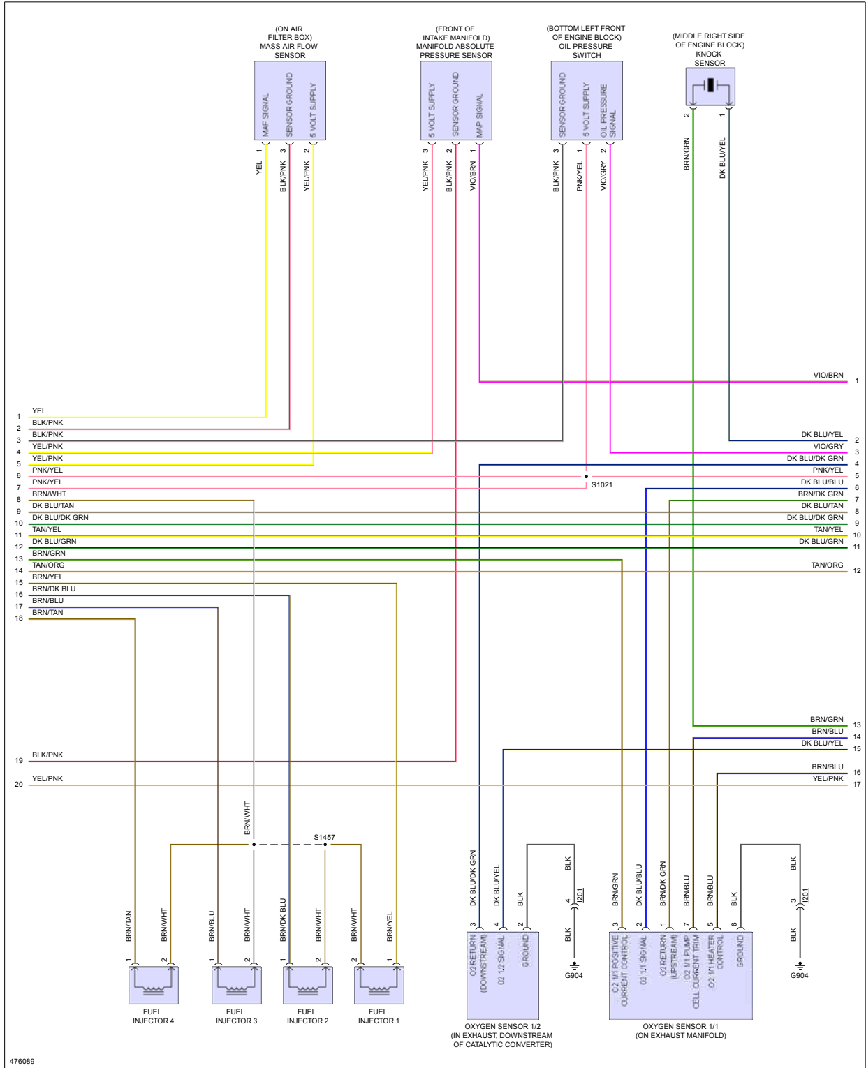
Fig 5: 2.4L, Engine Performance Circuit (5 of 6)
