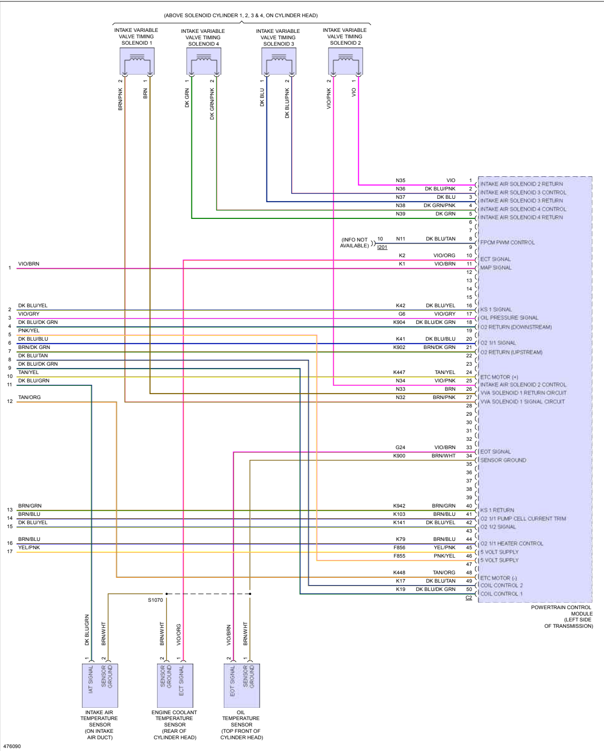
Fig 6: 2.4L, Engine Performance Circuit (6 of 6)
