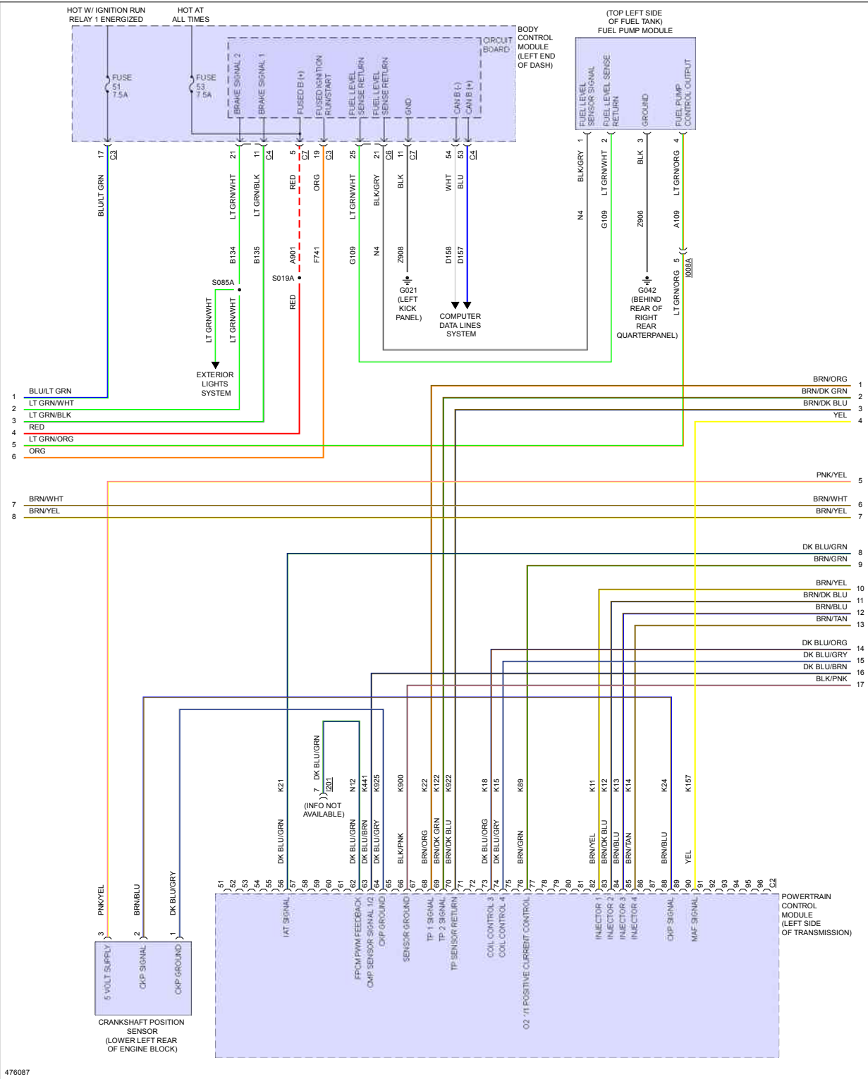
Fig 3: 2.4L, Engine Performance Circuit (3 of 6)
