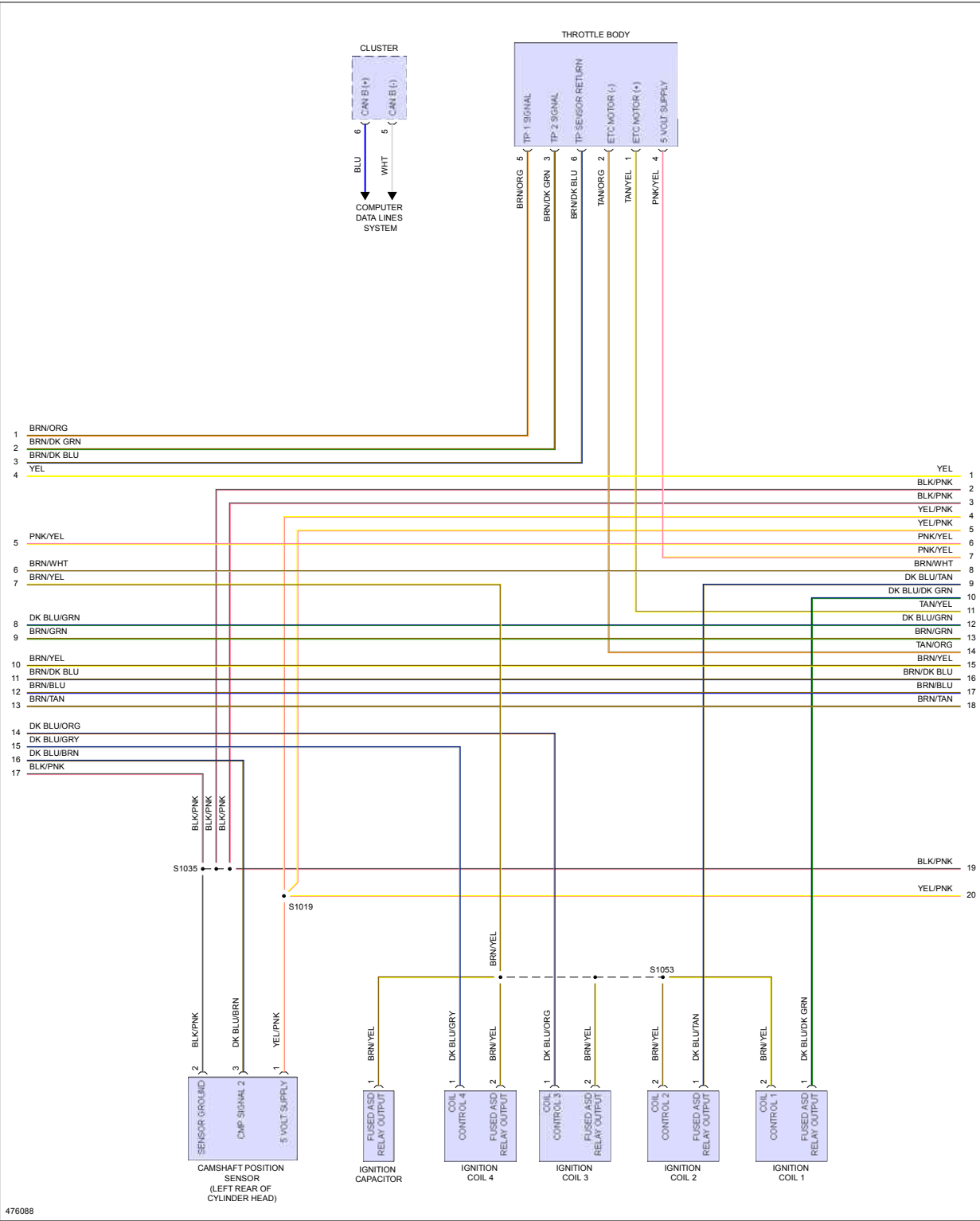
Fig 4: 2.4L, Engine Performance Circuit (4 of 6)
