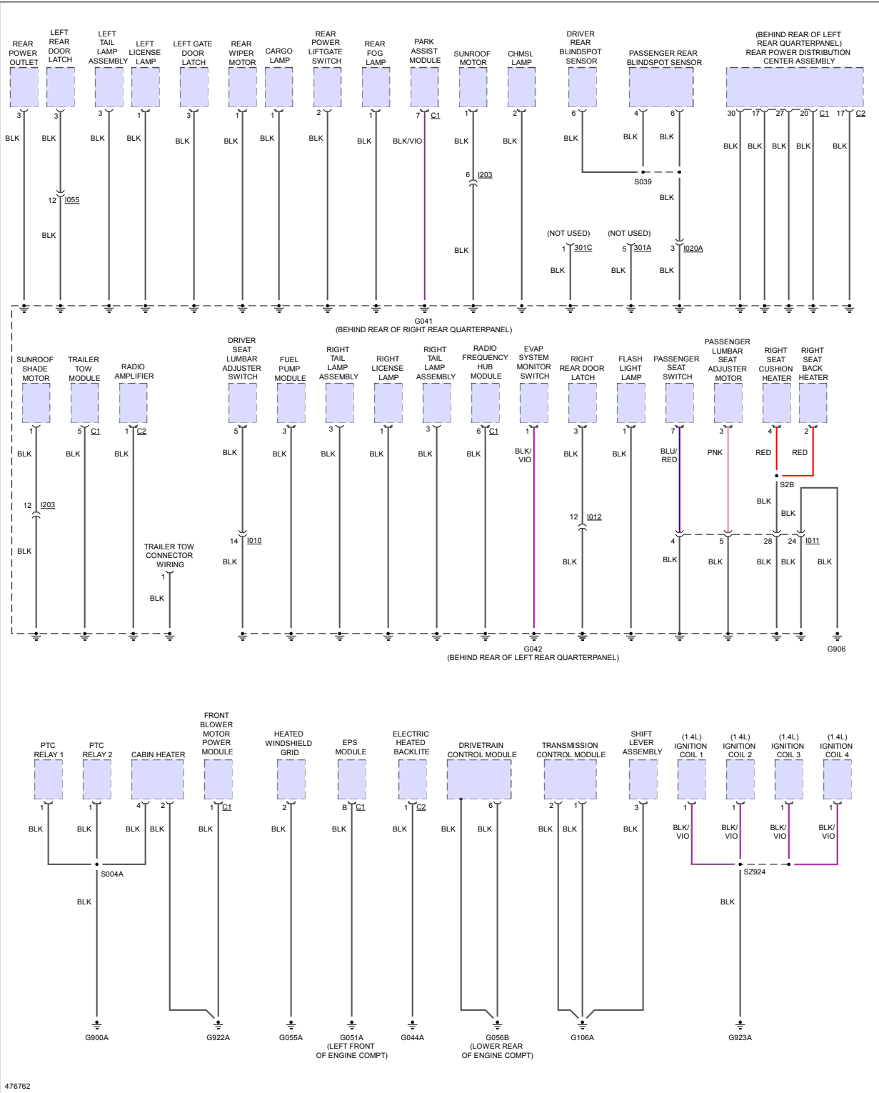
Fig 3: Ground Distribution Circuit (3 of 3)
