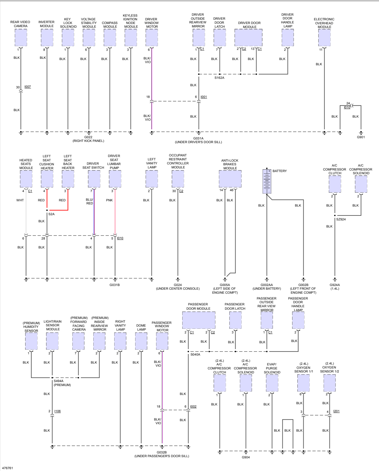
Fig 2: Ground Distribution Circuit (2 of 3)
