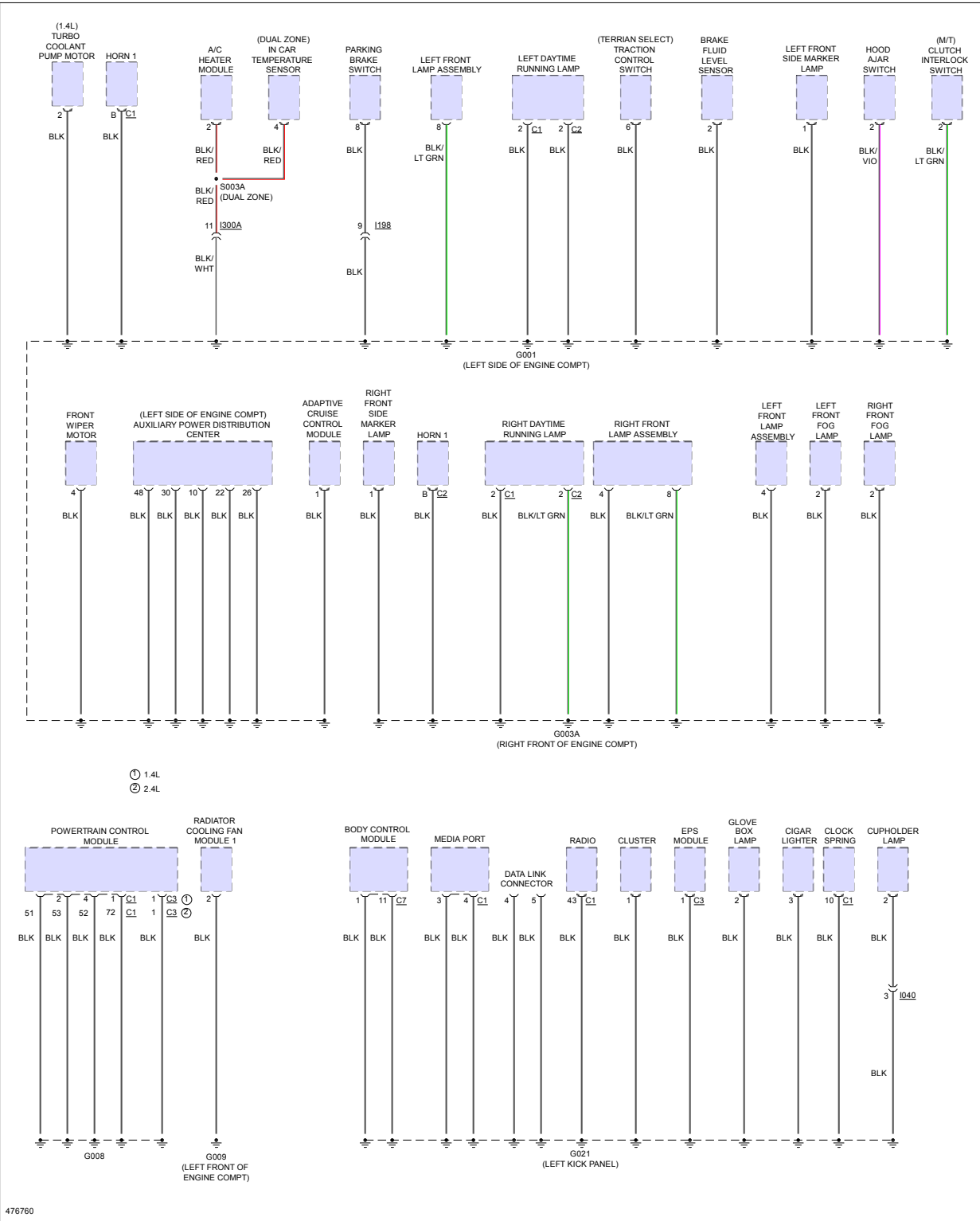
Fig 1: Ground Distribution Circuit (1 of 3)
