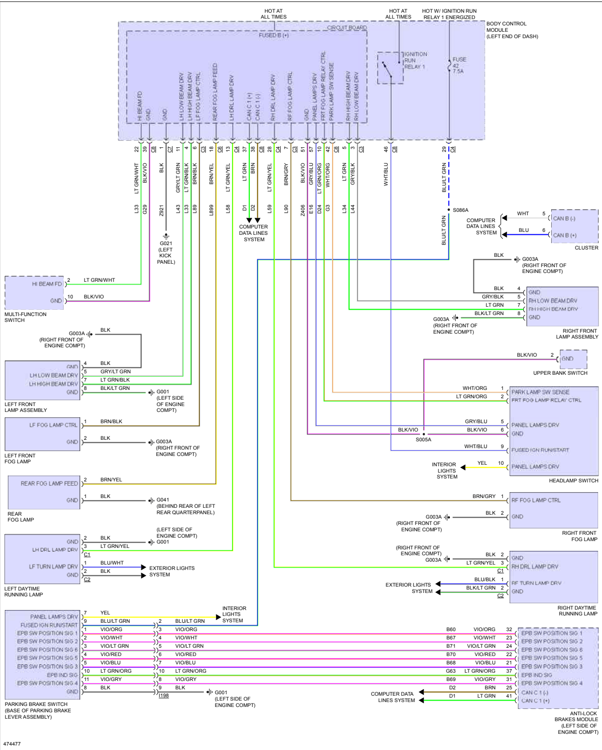
Fig 1: Headlights Circuit
