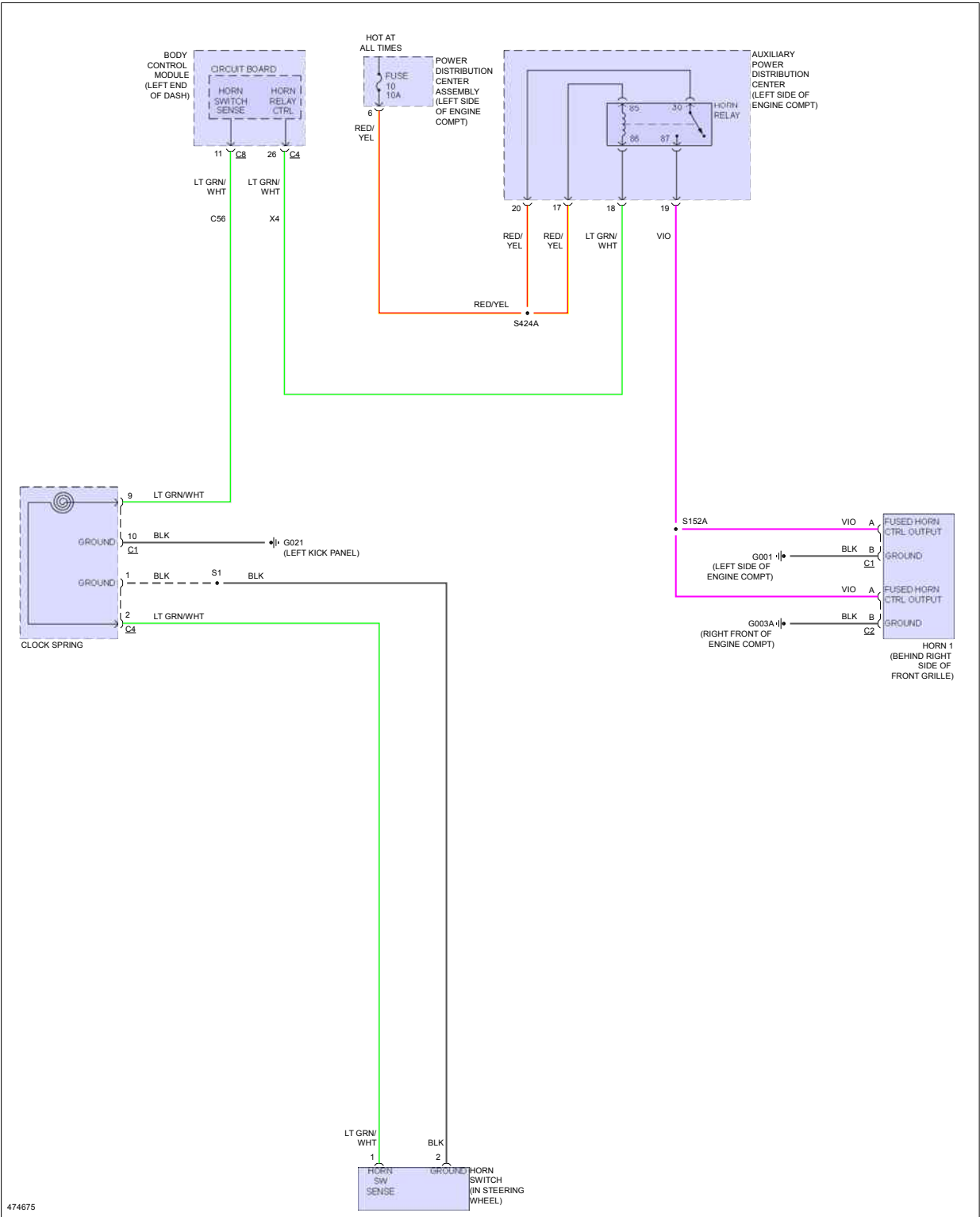
Fig 1: Horn Circuit
