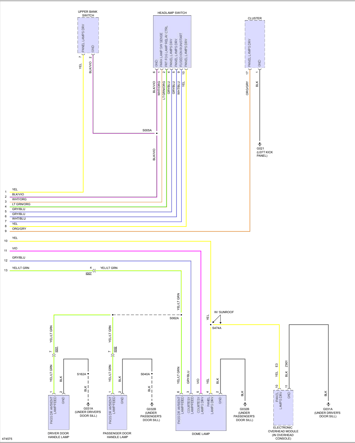
Fig 3: Interior Lights Circuit (3 of 3)
