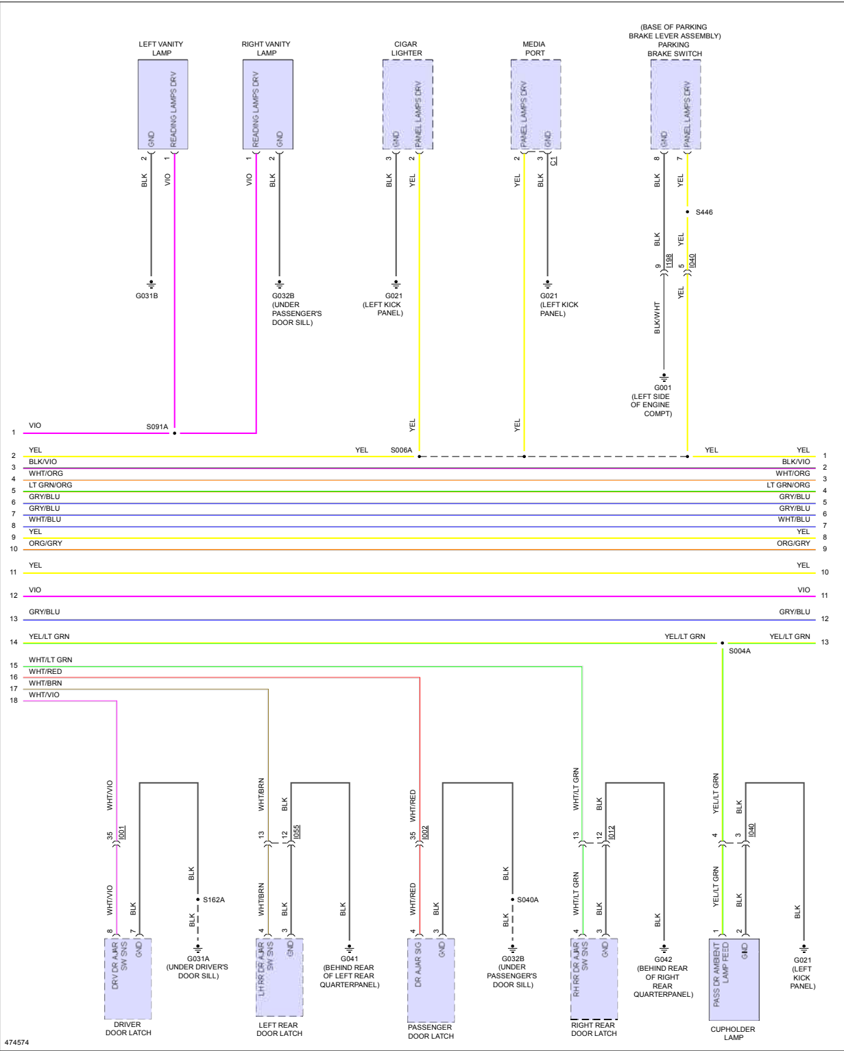
Fig 2: Interior Lights Circuit (2 of 3)
