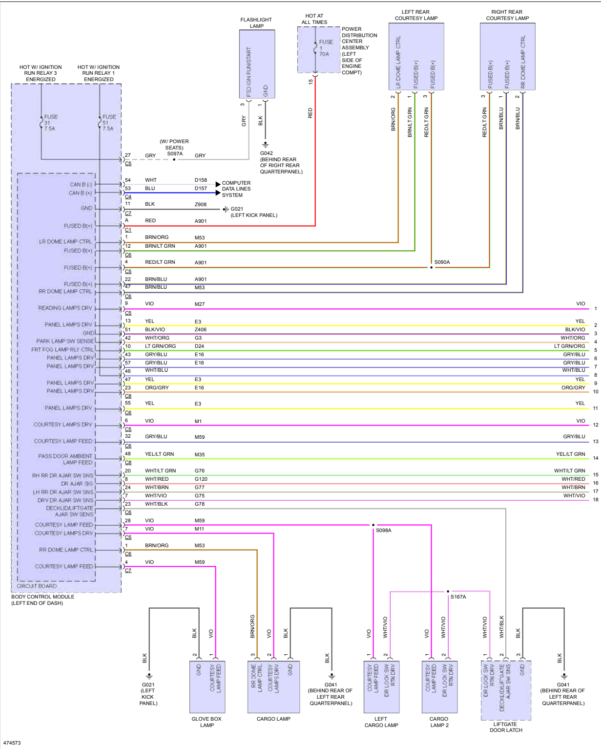
Fig 1: Interior Lights Circuit (1 of 3)
