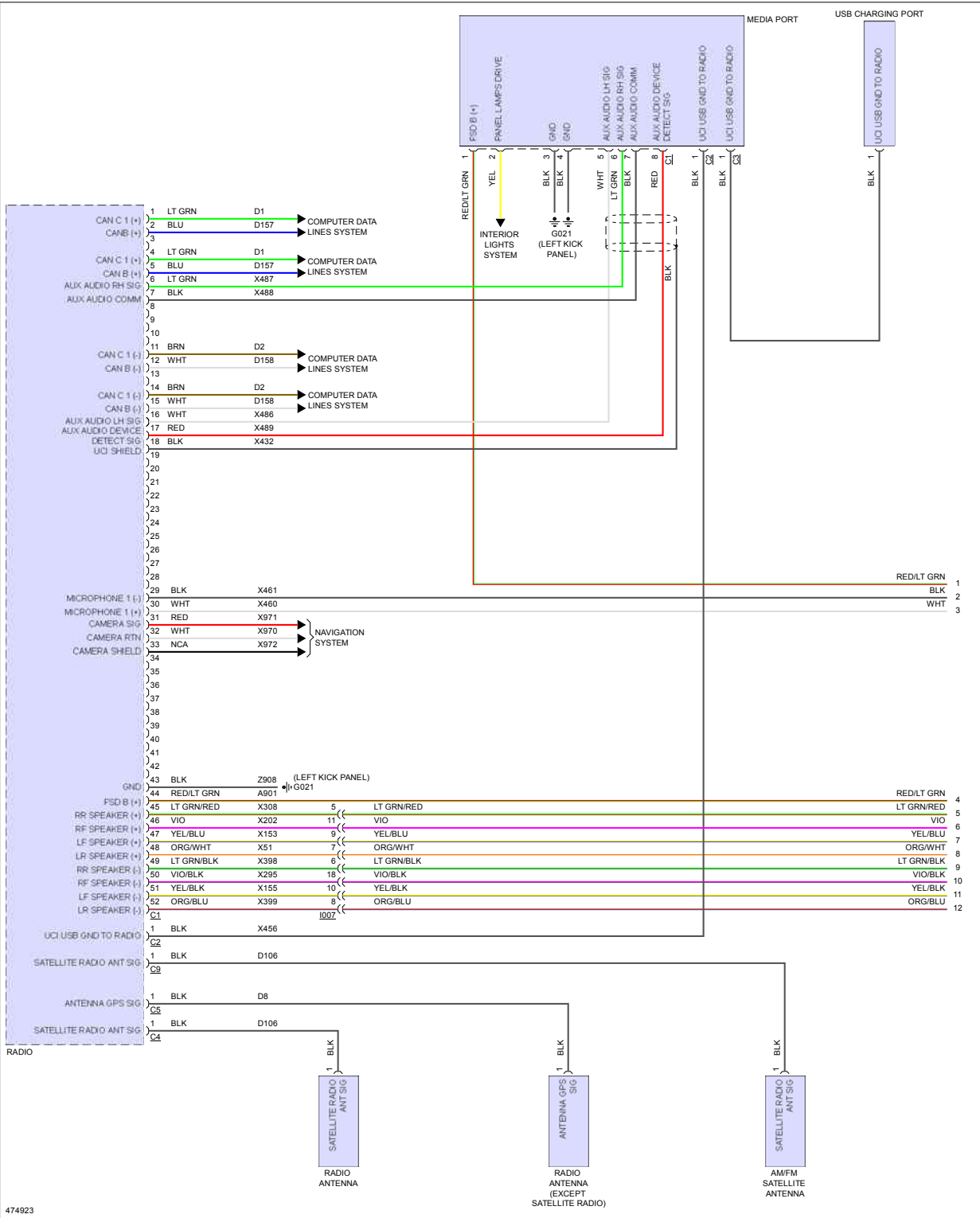
Fig 2: Navigation Circuit (1 of 3)
