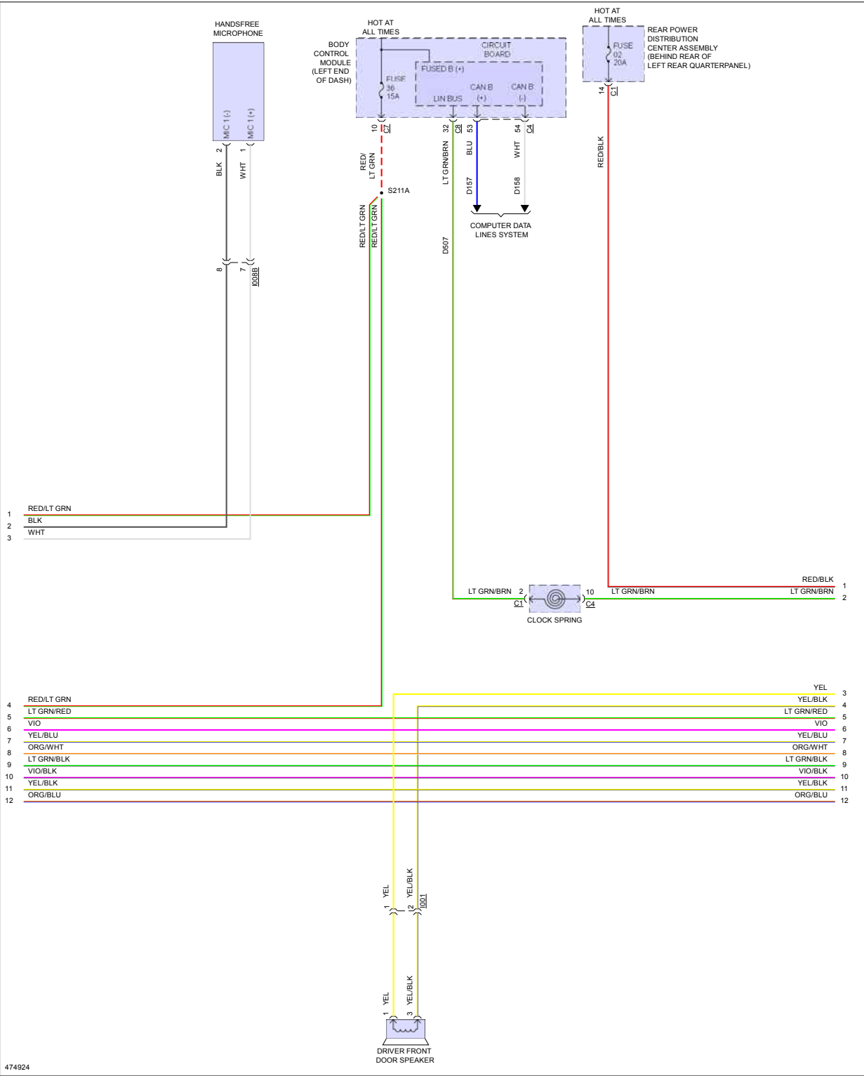
Fig 3: Navigation Circuit (2 of 3)
