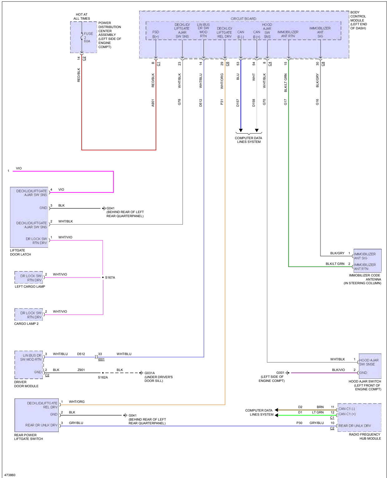
Fig 2: Power Door Locks Circuit (2 of 2)
