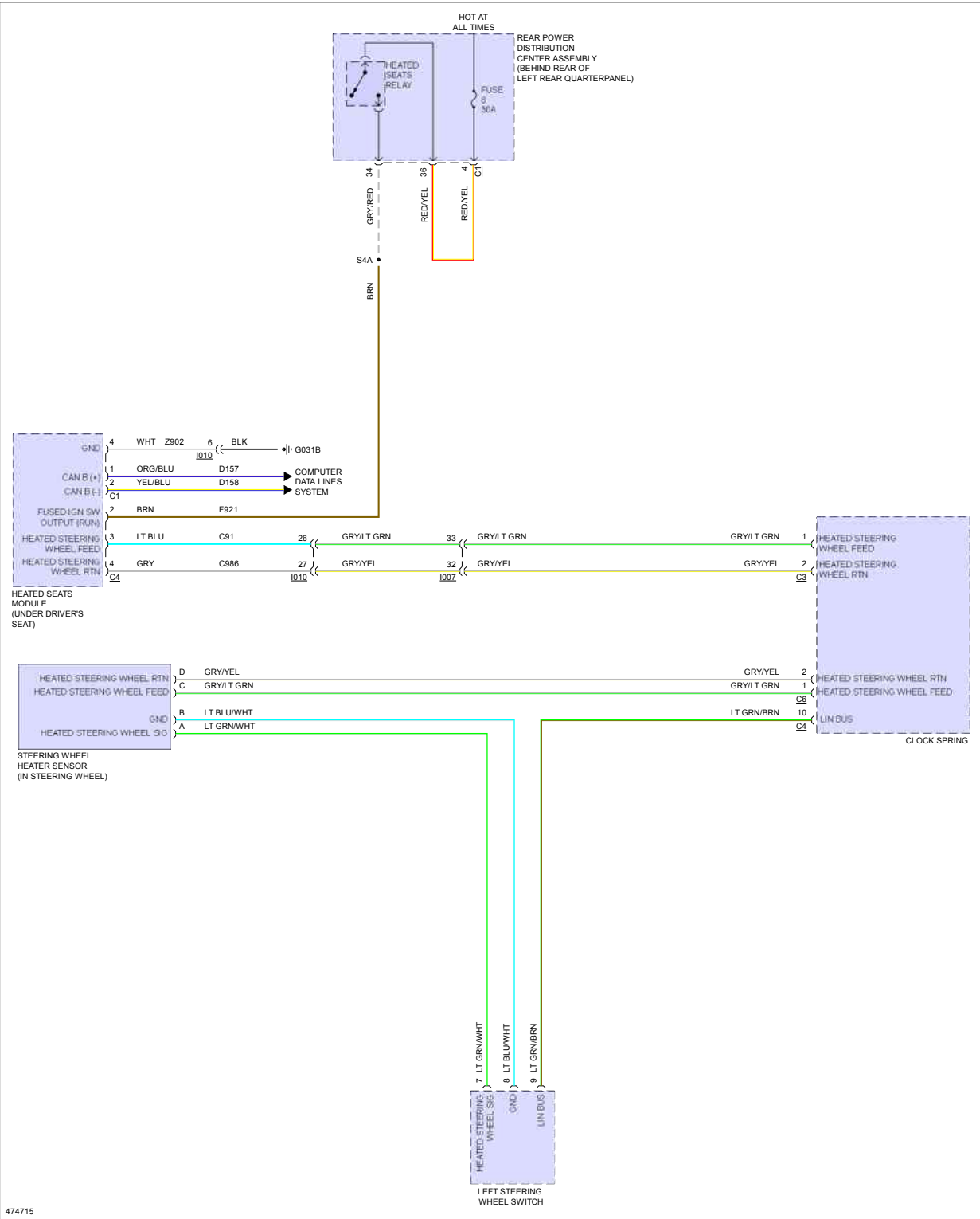
Fig 5: Heated Steering Wheel Circuit
