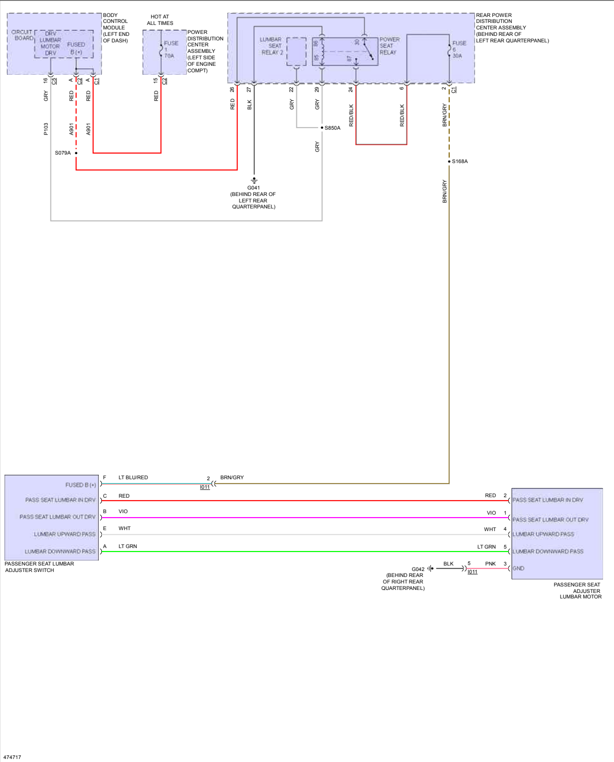
Fig 7: Passenger's Lumbar Circuit
