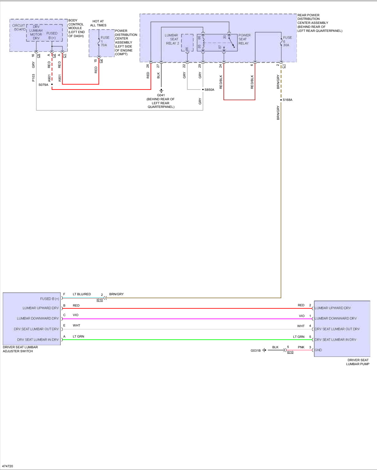
Fig 3: Driver"s Lumbar Circuit, Premium
