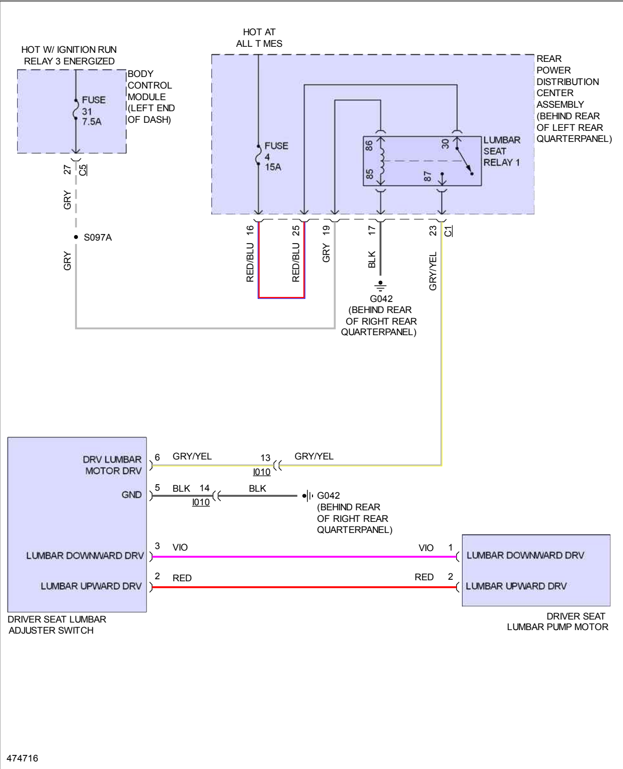
Fig 2: Driver"s Lumbar Circuit, Base
