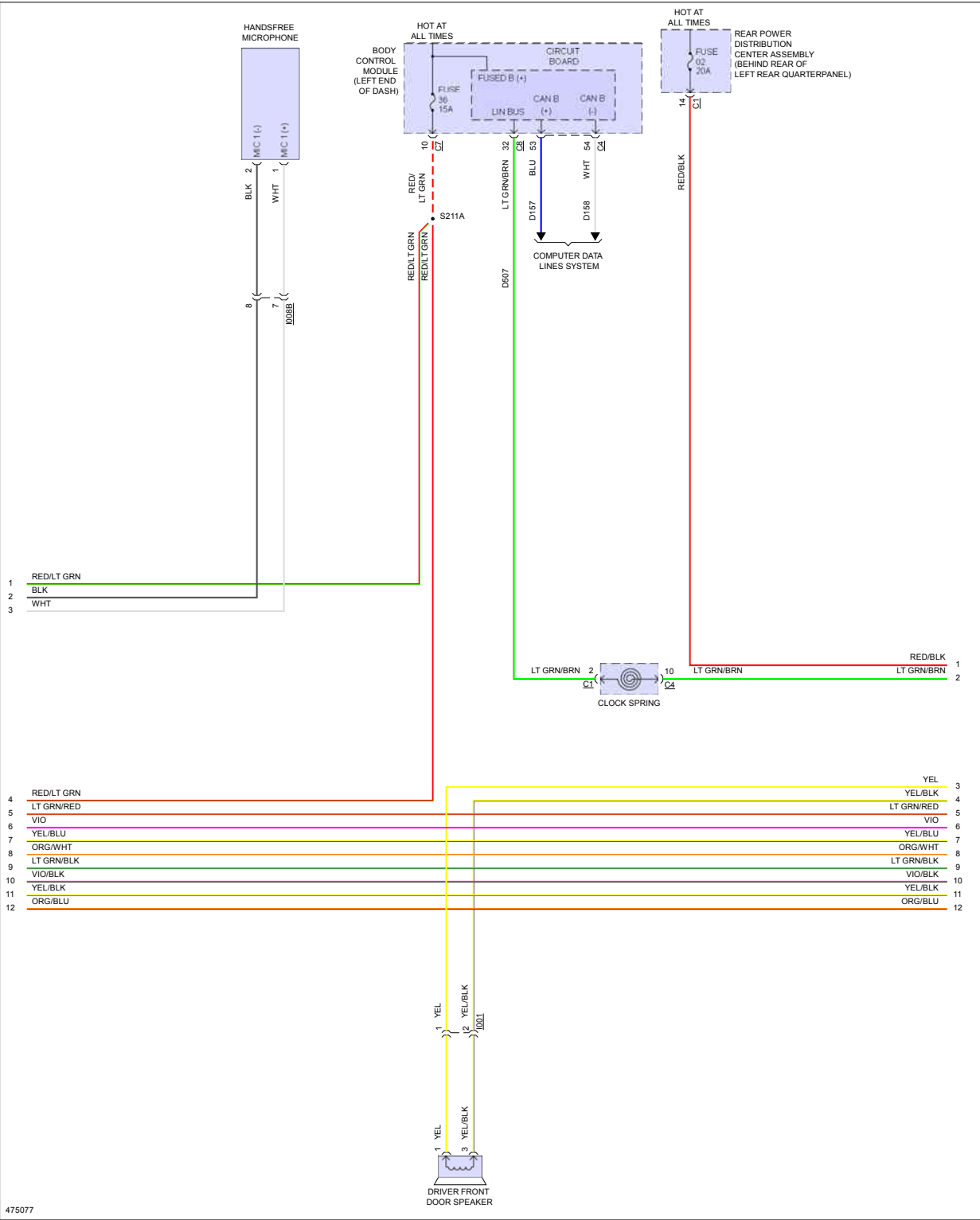
Fig 4: Radio Circuit, Premium (2 of 3)
