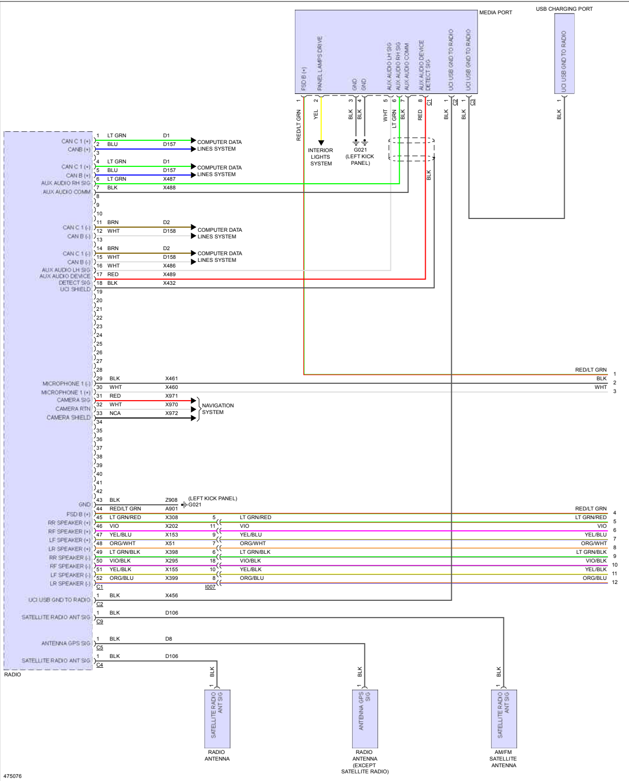
Fig 3: Radio Circuit, Premium (1 of 3)
