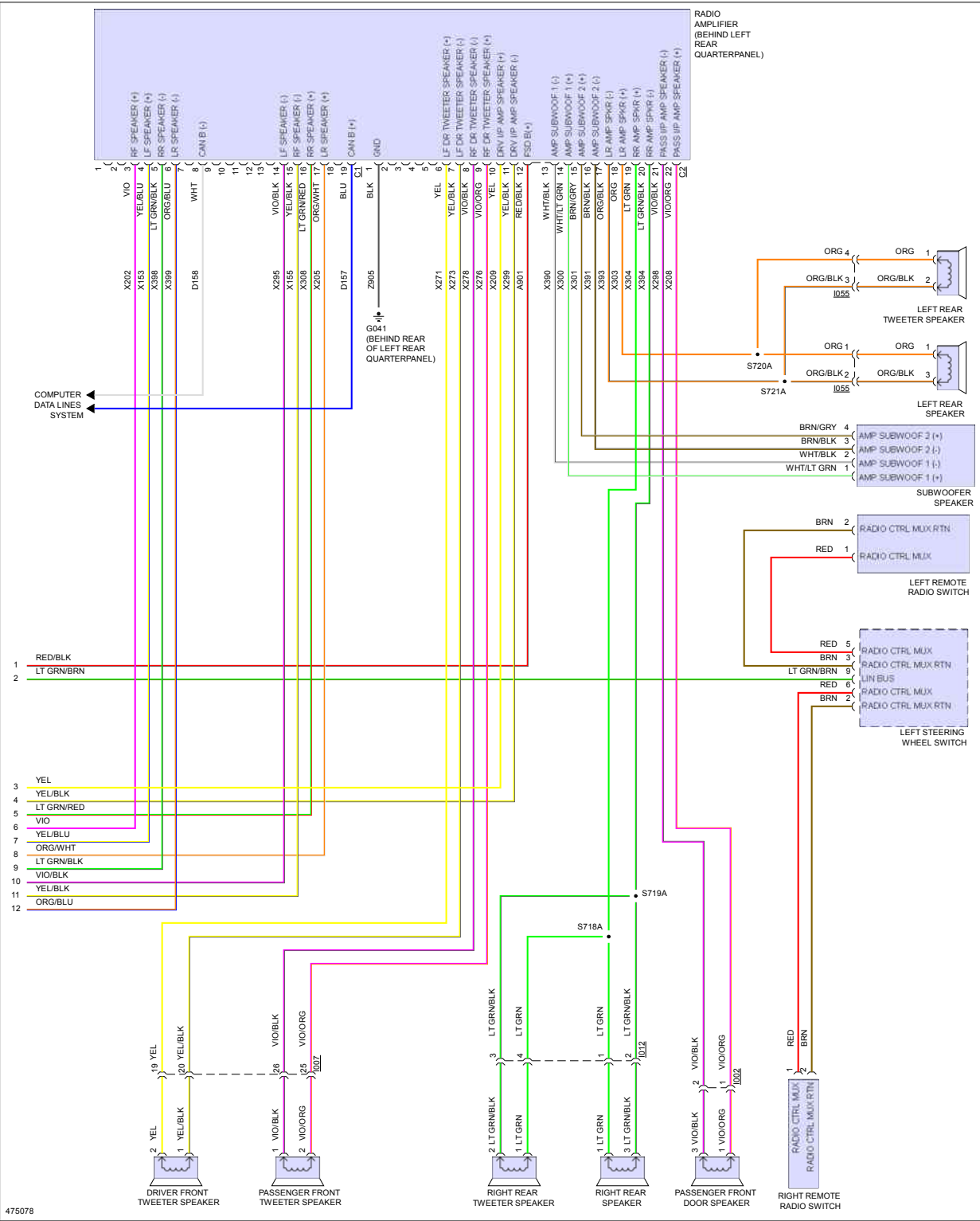
Fig 5: Radio Circuit, Premium (3 of 3)
