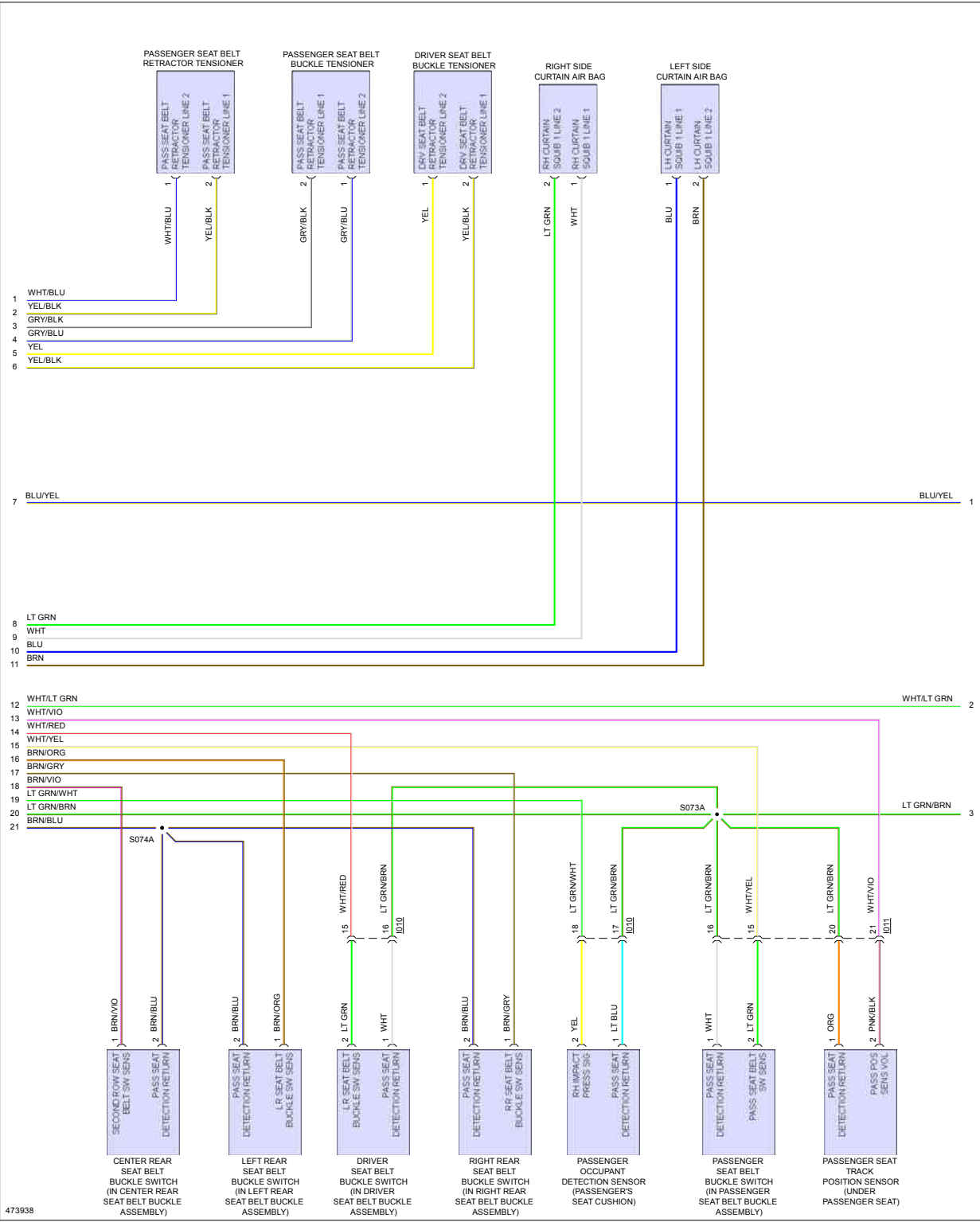
Fig 2: Supplemental Restraints Circuit (2 of 3)
