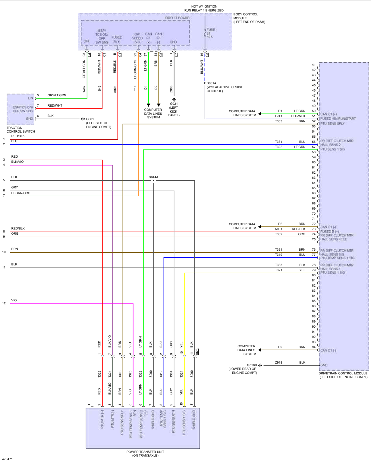
Fig 4: Transfer Case Circuit (2 of 2)
