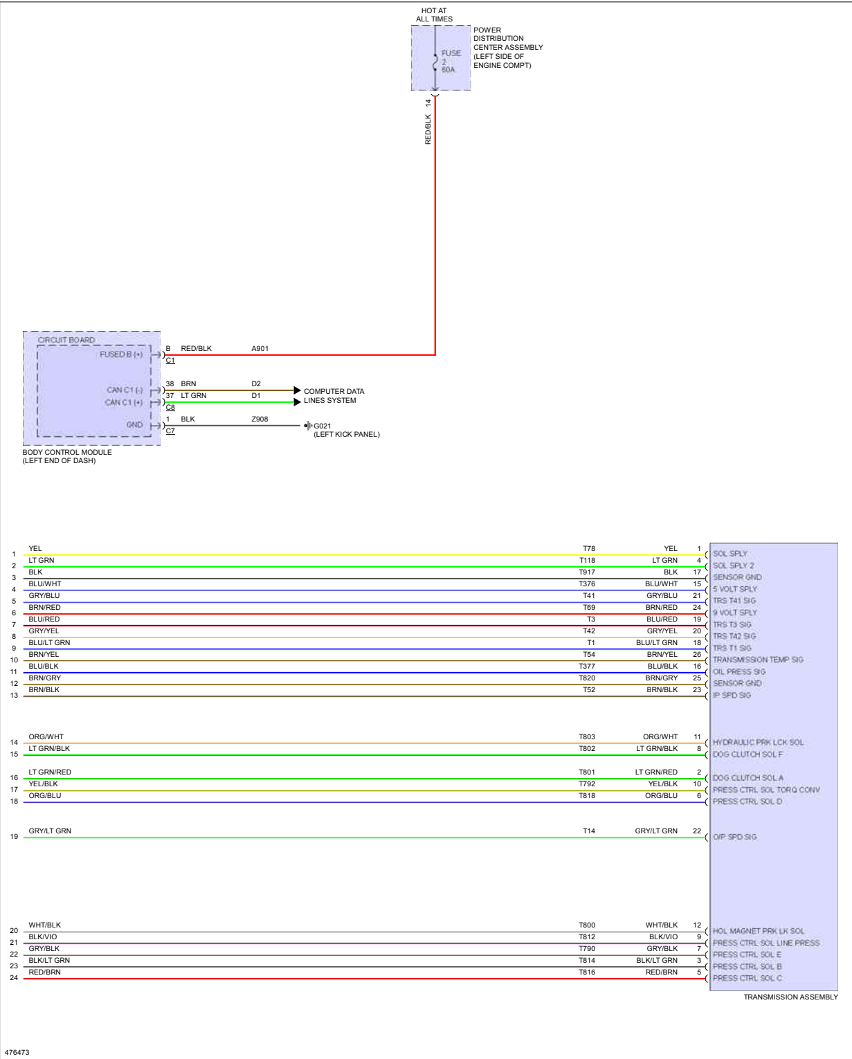
Fig 2: A/T Circuit (2 of 2)
