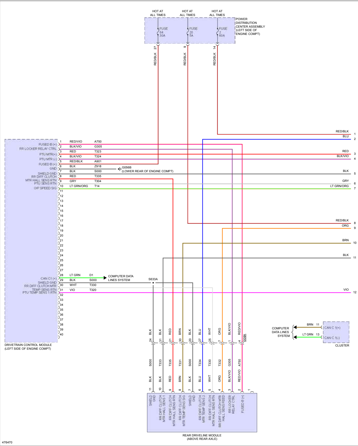
Fig 3: Transfer Case Circuit (1 of 2)
