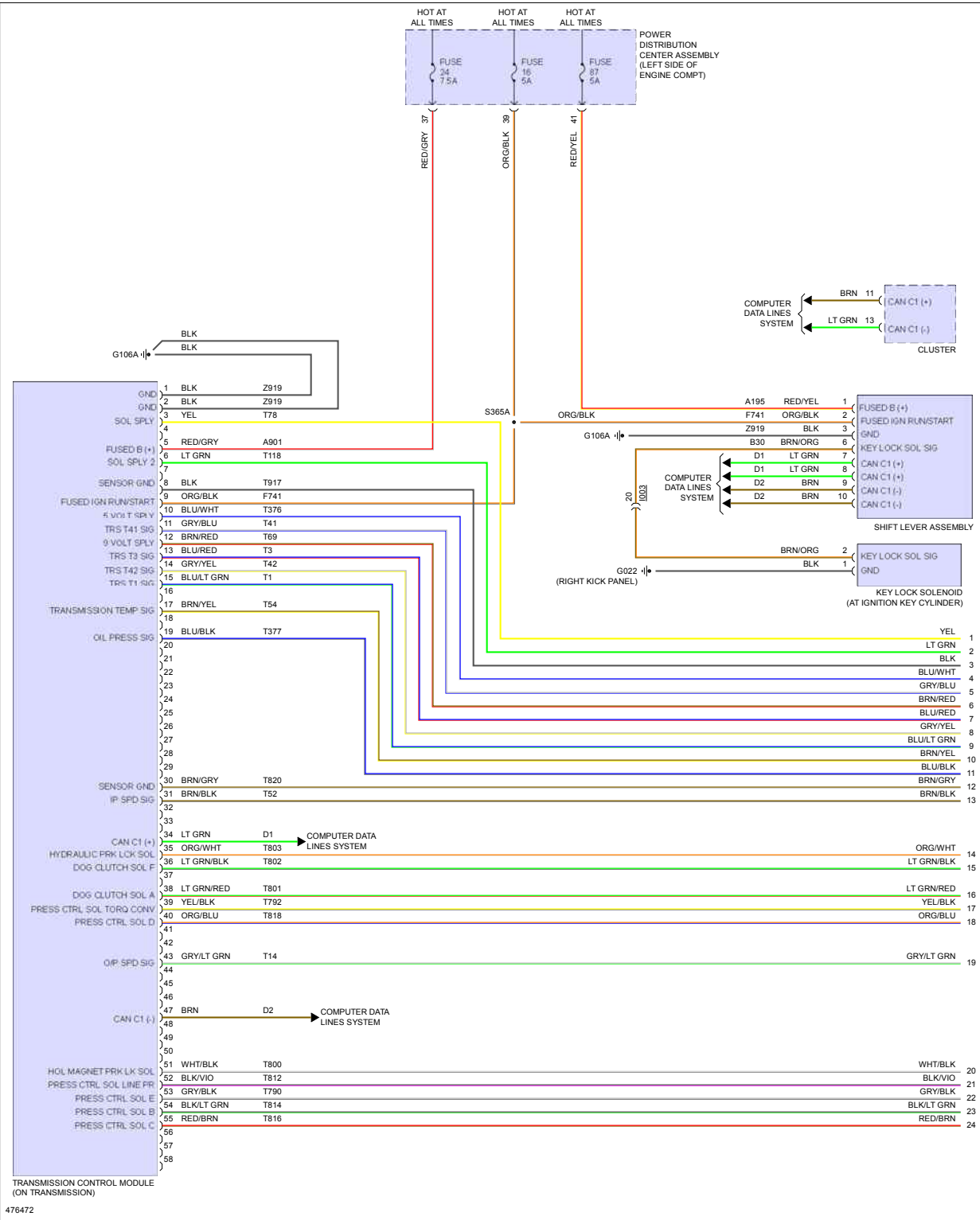
Fig 1: A/T Circuit (1 of 2)
