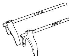
AISIN-900 Forks and Rails
